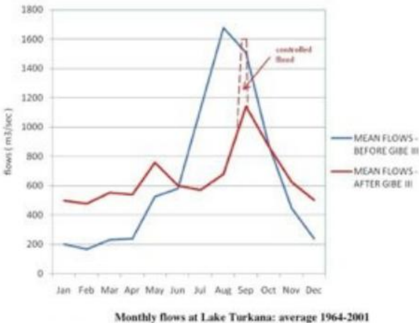
Figure 9: Mean monthly discharge of Omo before and after Gilgel Ghibe III dam (Source: EEPKO, Agriconsulting et al., 2009)
